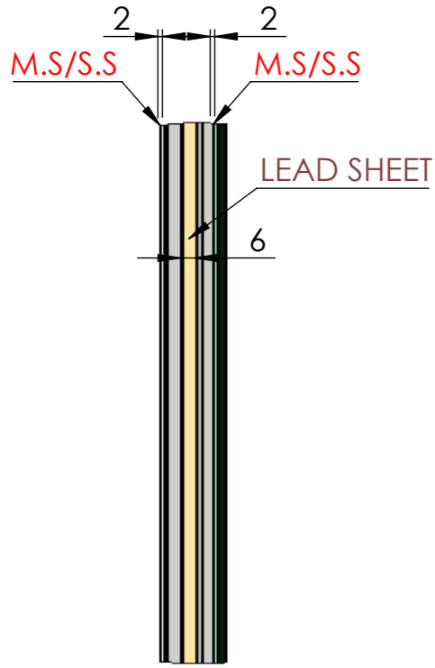
DETAIL F SCALE 1 : 3
