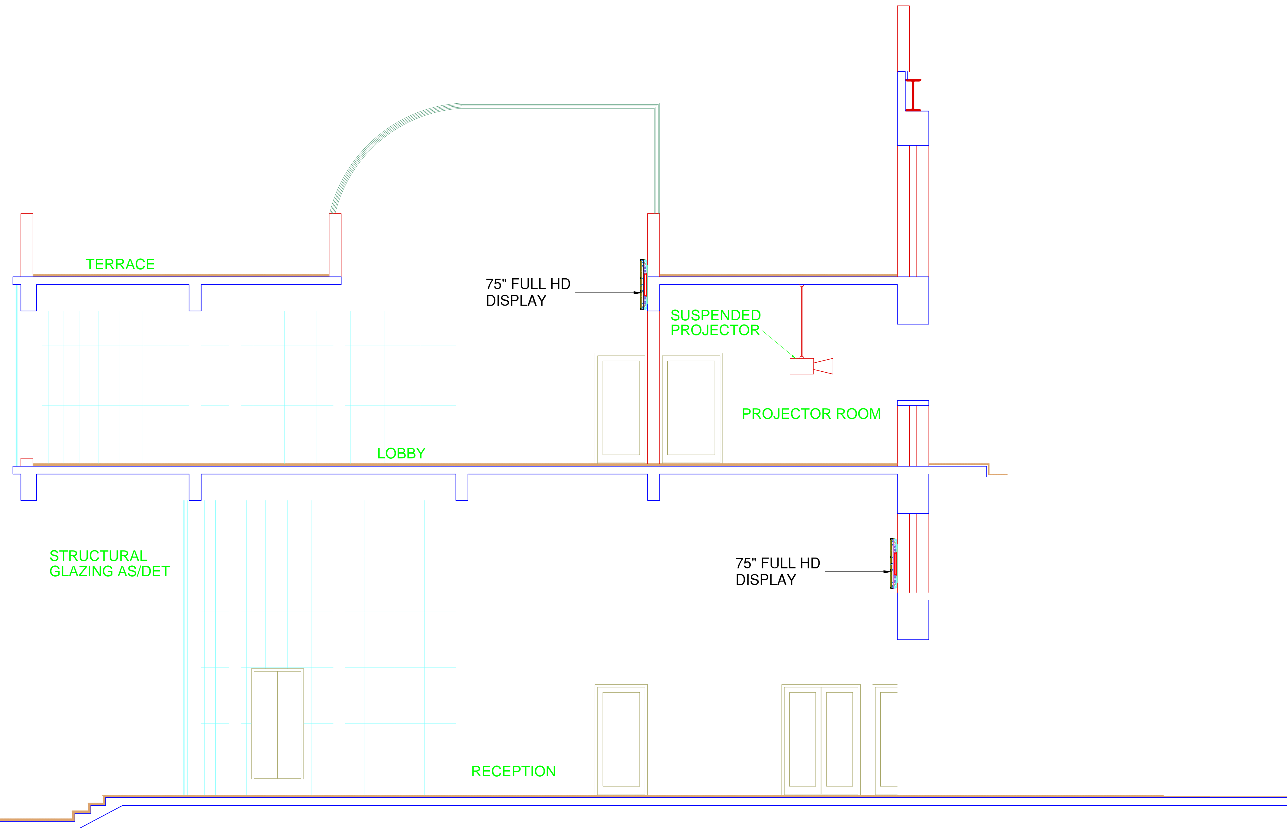
SECTION (Y-Y)
